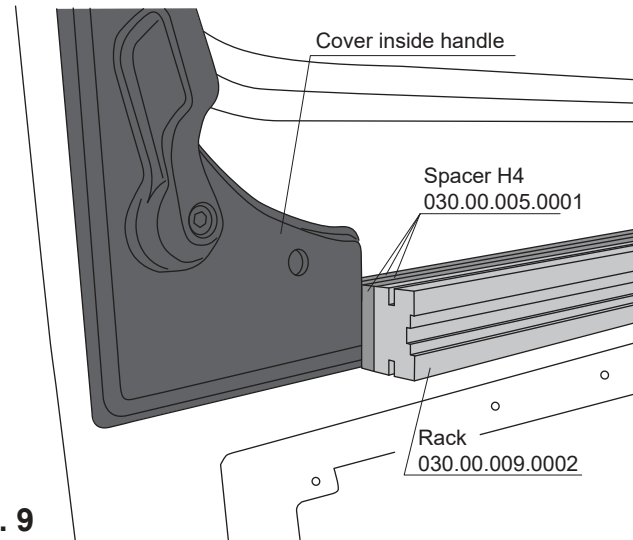
INSTALLATION VARIANT FOR SPACER H4 AND RACK UP TO THE COVER OF THE INSIDE HANDLE
