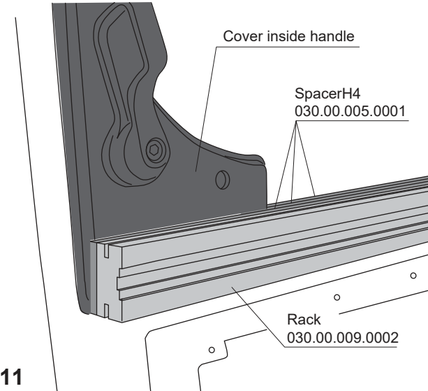
INSTALLATION VARIANT FOR SPACER H4 AND RACK UP TO DOOR EDGE
