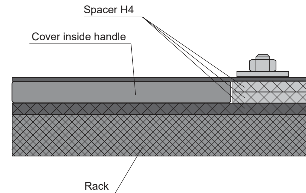
INSTALLATION VARIANT FOR SPACER H4 AND RACK UP TO DOOR EDGE
